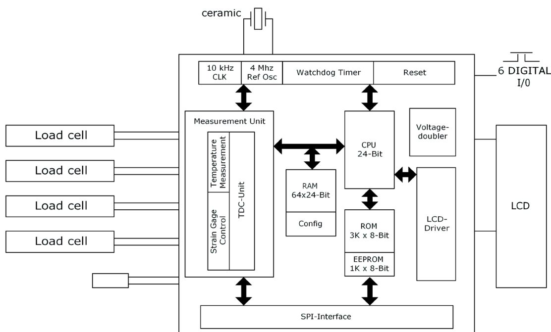
Figure 1.1 Block Diagram
