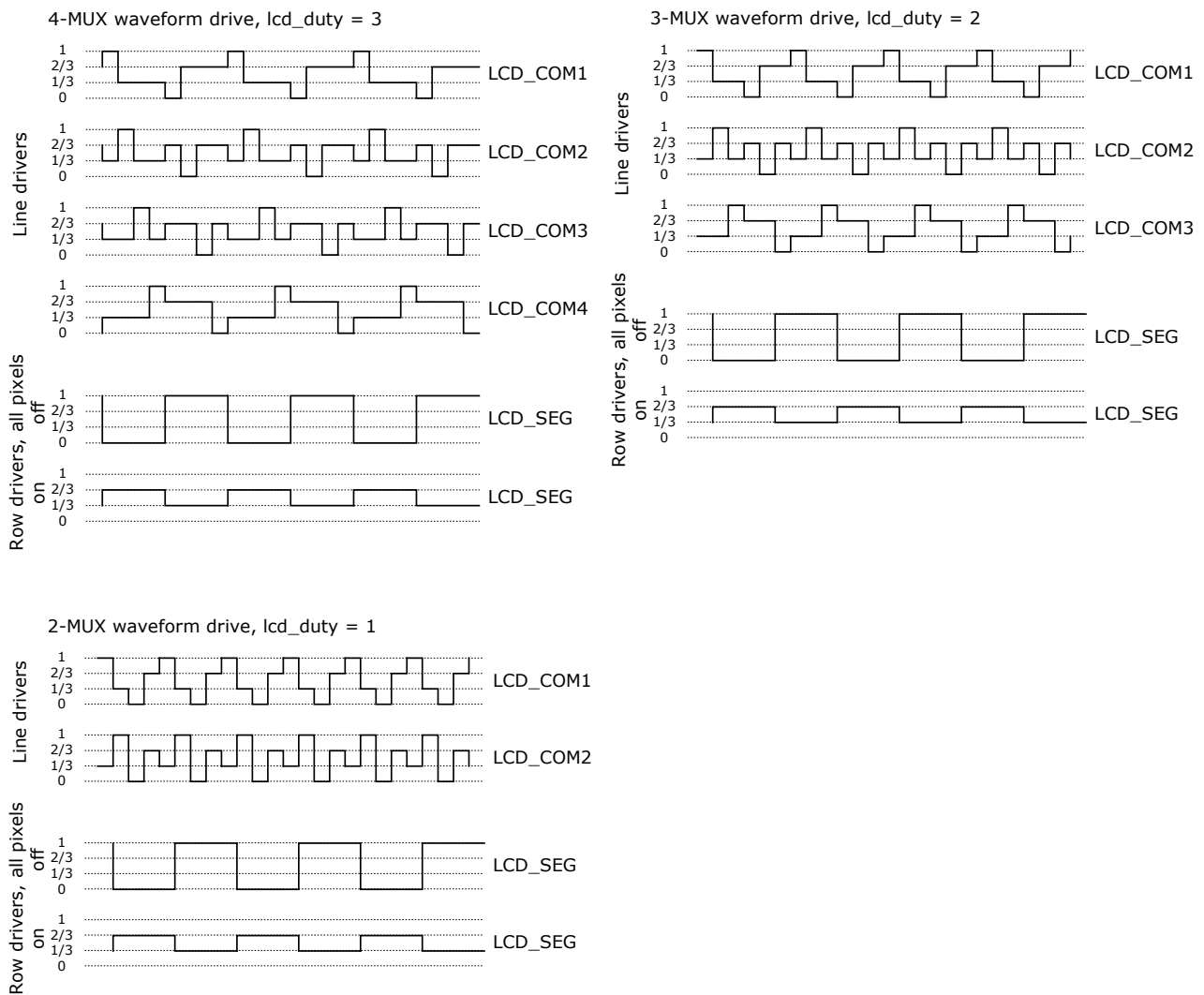
Figure 4.4 LCD driving
