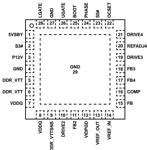
ISL6537 (6x6 QFN)
