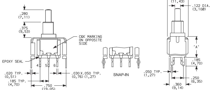
8261SH9_BE2 DPDT
