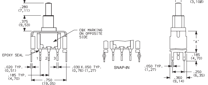
8161SH9_BE2 SPDT
