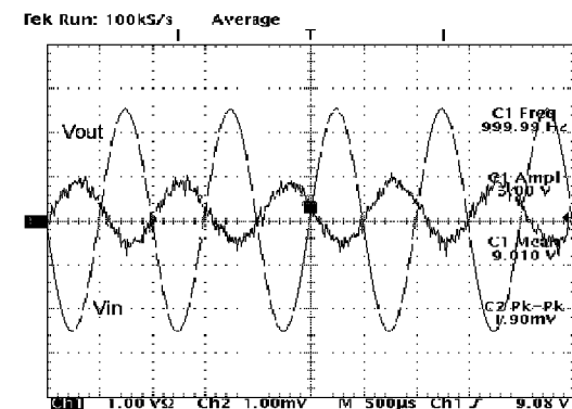
Supply Voltage Rejection at V_{OUT} = 5V
