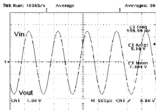
Supply Voltage Rejection at V_{OUT} = 2.85V
