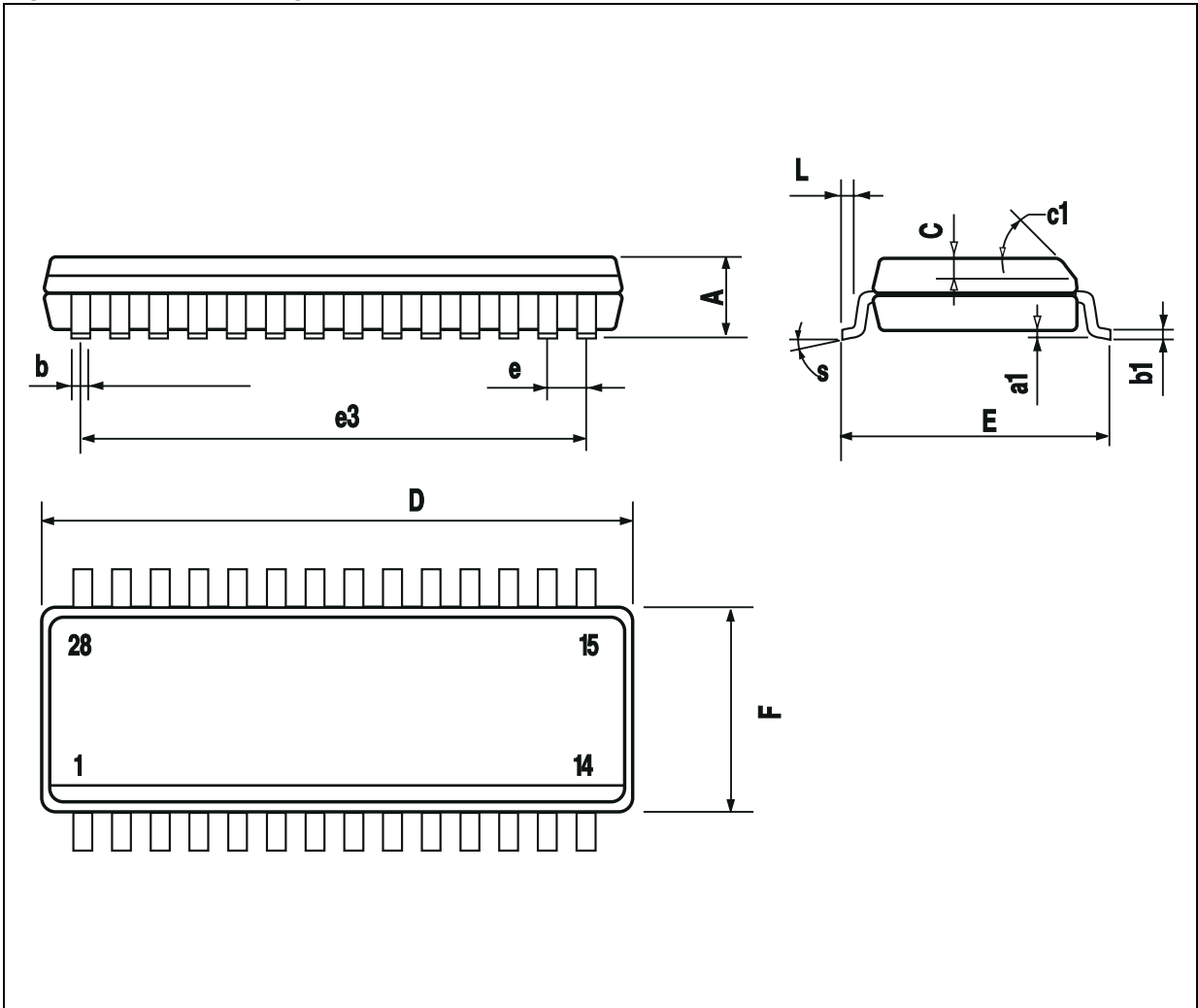
Figure 46. SO-28 Package Dimensions
