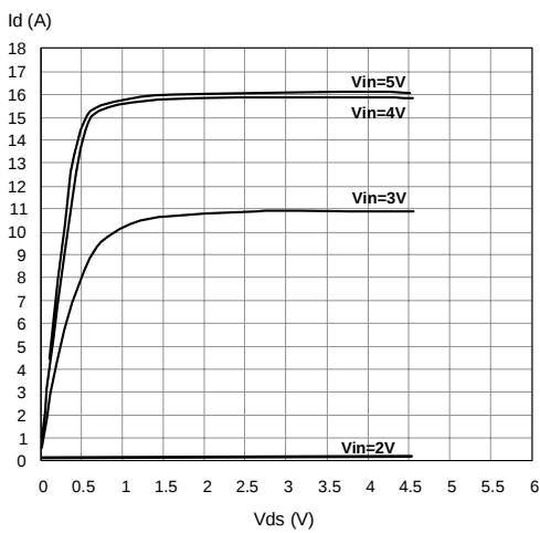
Figure 33. Output Characteristics
