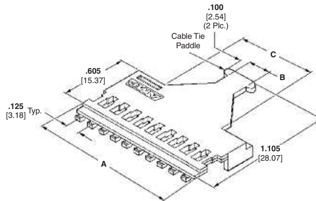
Cover 103349 Series with Wide Cable Tie Paddle
