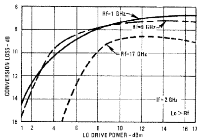
Conversion Loss vs. LO Drive Power
