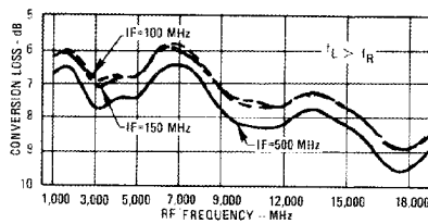
Conversion Loss vs. Frequency LO @ +13 dBm
