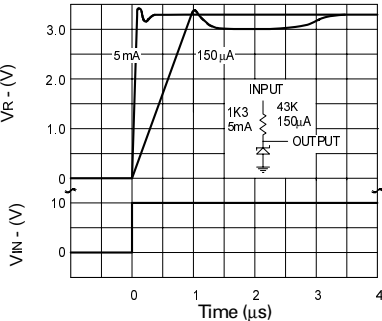
Transient Response (Repetitive Pulse)
