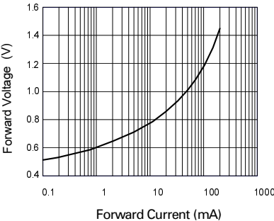
Forward Characteristics
