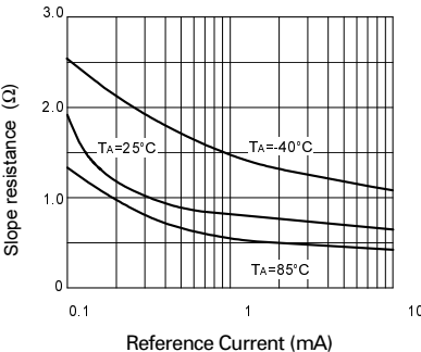
Slope Resistance v Current
