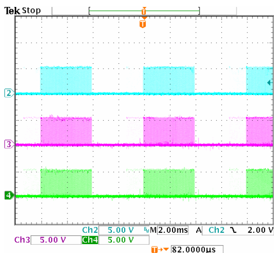
Figure 6- Gate signals during digital dimming with 50% duty cycle CH2= A_{OUT}(\text{Master}) , CH3= A_{OUT}(\text{Slave1}) , CH4= A_{OUT}(\text{Slave2})
