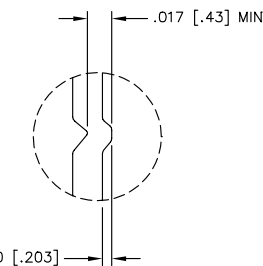
CRIMP DETAIL
