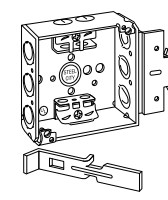
52151 MS X* MS bracket for 1/2", 3/4", 4" metal studs
