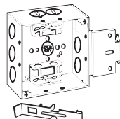
52171 MSX* MS bracket for 1/2", 3/4", 4" metal studs
