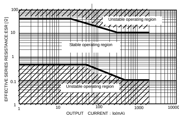
Fig.34 ESR vs. Io Characteristics (BAxxDD0)
