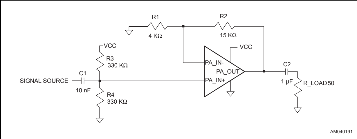
Figure 3. PA linearity test circuit
