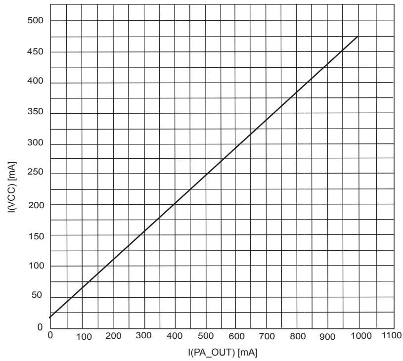
Figure 4. I(VCC) vs. I(PA_OUT) curve - typical values
