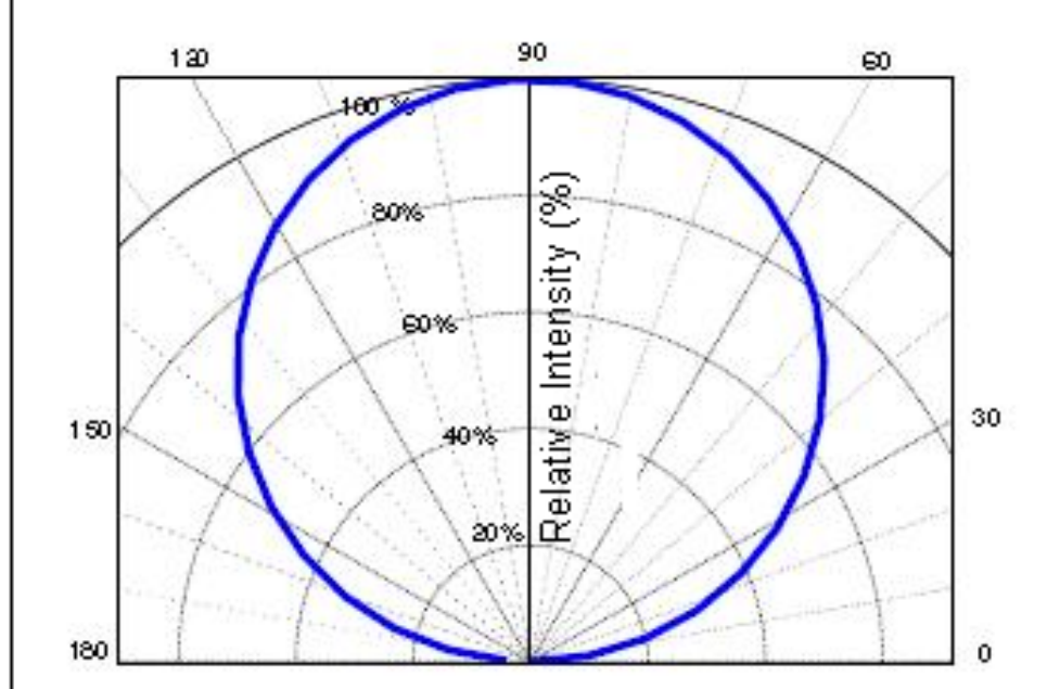
Figure 3: Typical Polar Radiation Pattern
