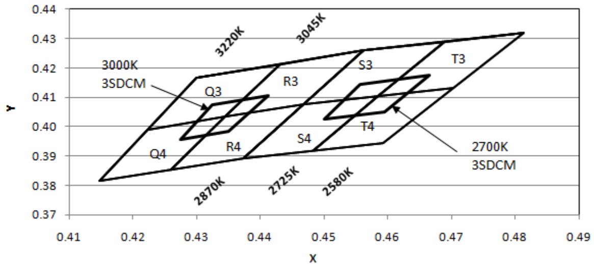
Figure 16: Graph of Warm White Test Bins in xy Color Space
