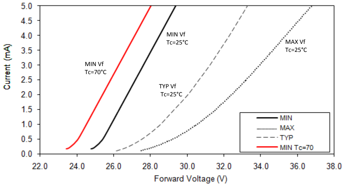
Figure 13: Current vs. Voltage, BXRA-W5700, BXRA-N6300 and BXRA-C8000
