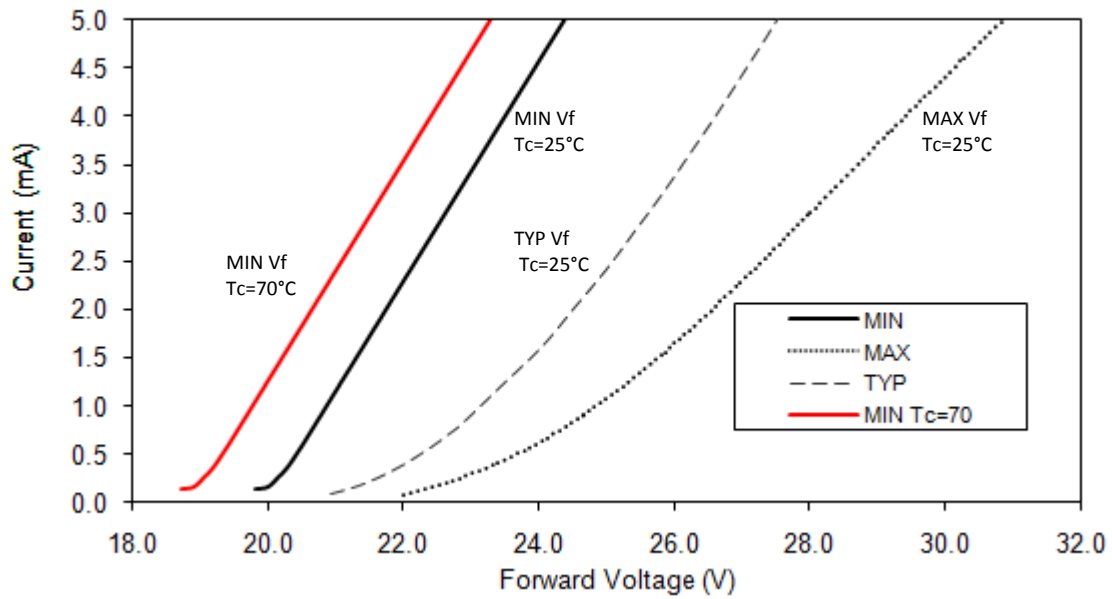
Figure 12: Current vs. Voltage, BXRA-W3500, BXRA-N4000 and BXRA-C5000
