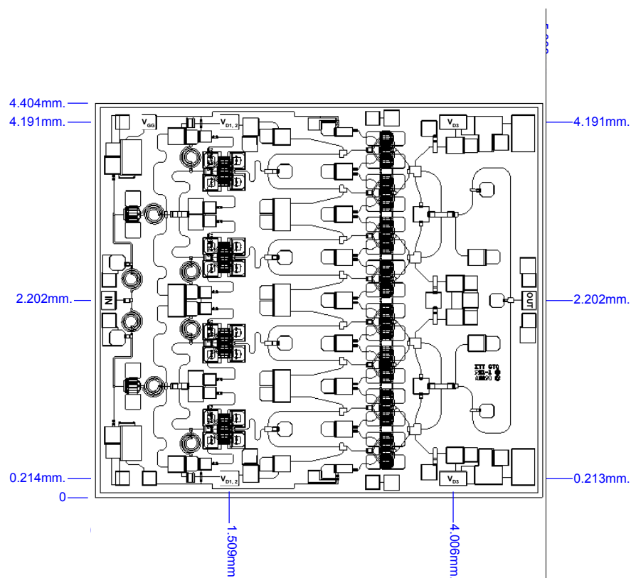
Figure 5. Die Layout
