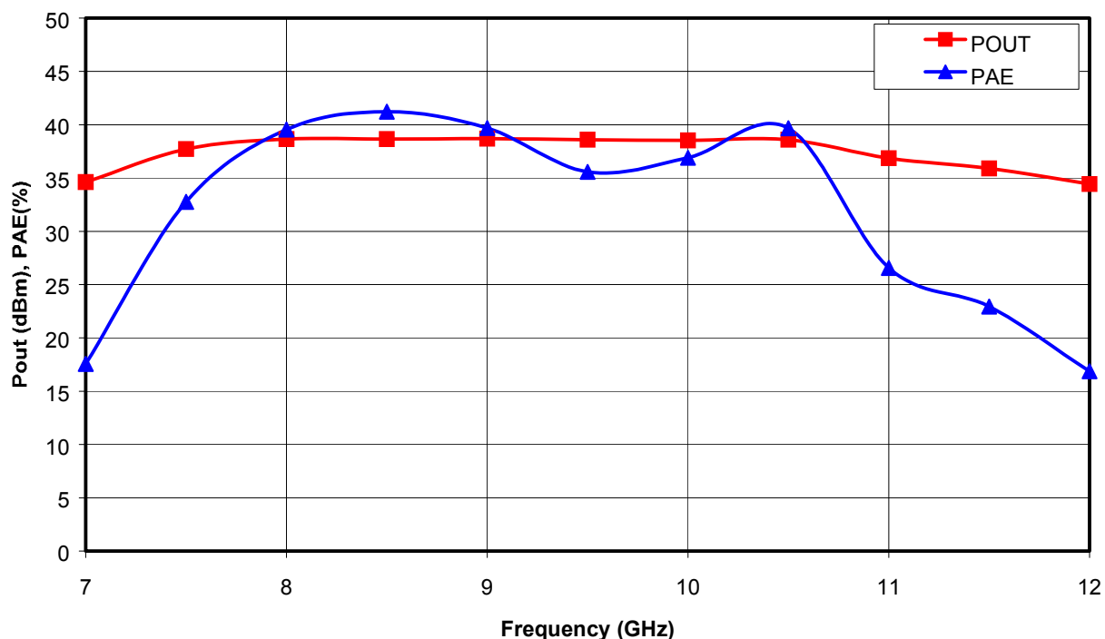
Figure 1. Output Power and Power Added Efficiency vs. Frequency at V_{DD} = 8V , P_{in} = 20 dBm.
