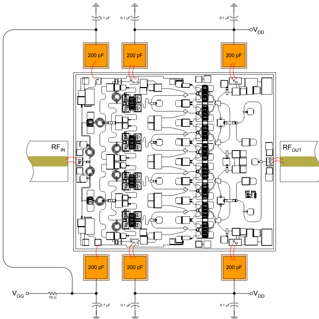
Figure 6. Recommended bonding diagram for pedestal mount. Support circuitry typical of MMIC characterization fixture for CW testing.
