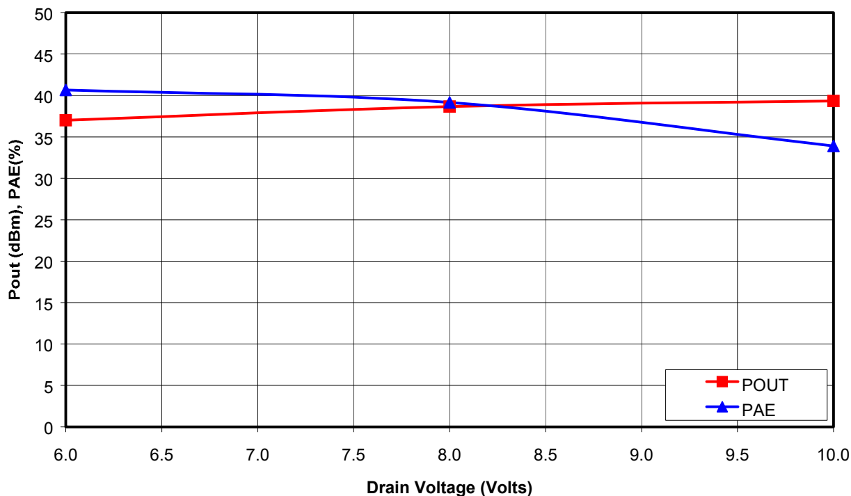
Figure 2. Saturated Output Power and Power Added Efficiency vs. Drain Voltage at f_0 = 9 GHz.
