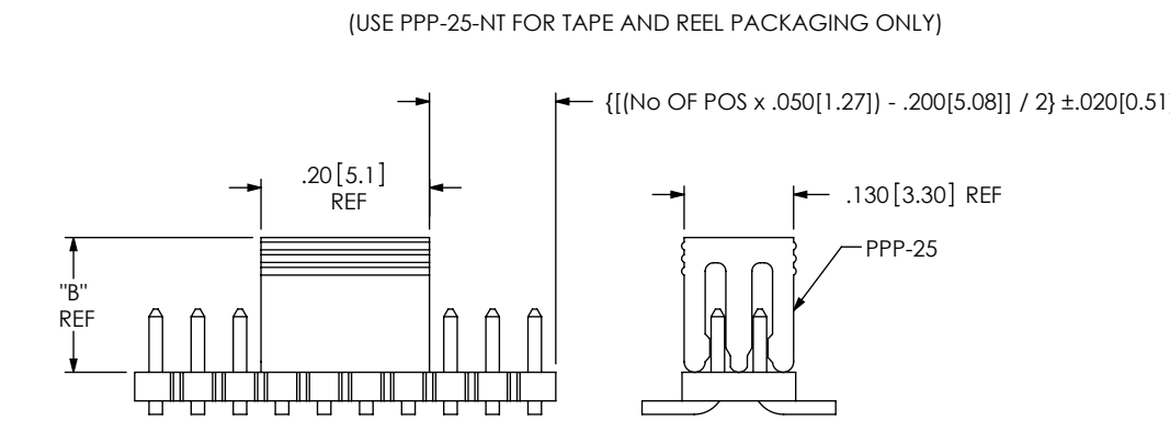
FIG 5 -DV-P OPTION FTS-110-02-XX-DV-P SHOWN (DIFFERENT AS SHOWN, OTHERWISE SAME AS FIG 1)
