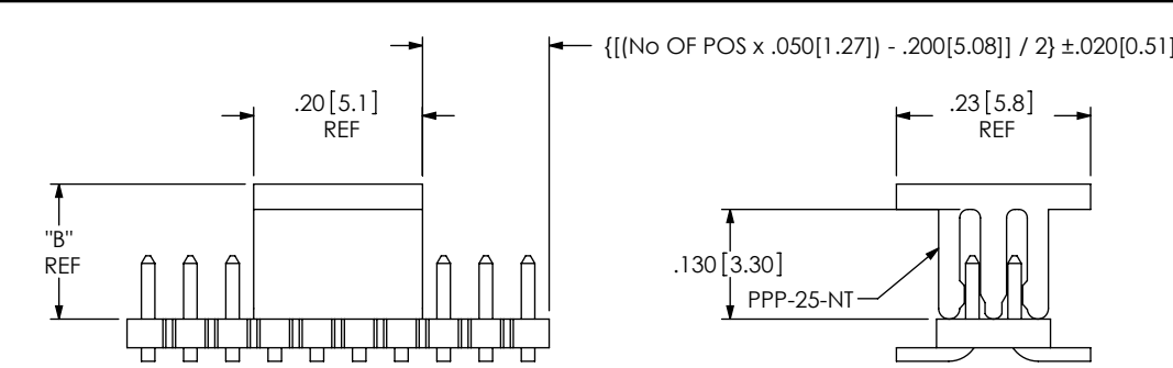
FIG 3 -DV-S OPTION (SEE NOTES 6 & 7) FTS-110-02-XX-DV-S SHOWN (DIFFERENT AS SHOWN, OTHERWISE SAME AS FIG 1)
