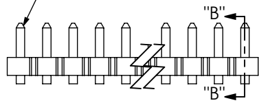
FIG 2 FTS-1XX-03-XX-DV SHOWN (DIFFERENT AS SHOWN, OTHERWISE SAME AS FIG 1)
