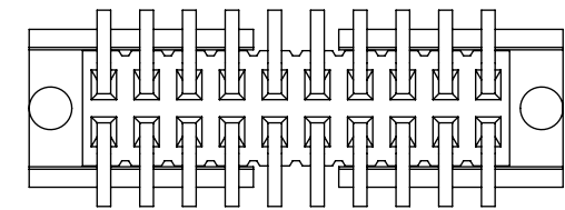
FIG 4 -DV-SA OPTION (SEE NOTES 6 & 7) FTS-106-02-XX-DV-SA SHOWN (DIFFERENT AS SHOWN, OTHERWISE SAME AS FIG 1)
