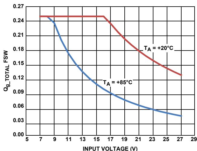
FIGURE 28. ALLOWED MAXIMUM GATE CHARGE vs INPUT VOLTAGE
