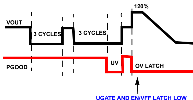
FIGURE 19. PGOOD TIMING UNDER UV AND OV
