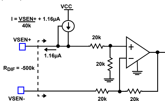
FIGURE 31. EQUIVALENT DIFFERENTIAL AMPLIFIER
