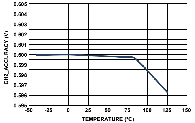
FIGURE 3. CHANNEL 2 ACCURACY vs TEMPERATURE
