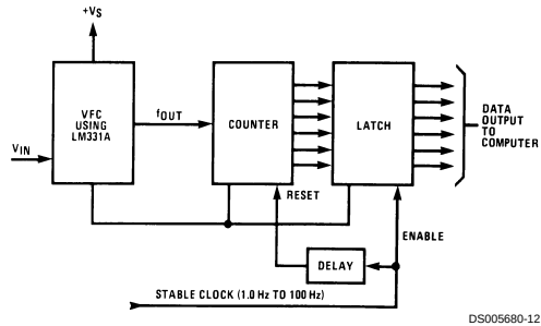
Basic Analog-to-Digital Converter Using Voltage-to-Frequency Converter
