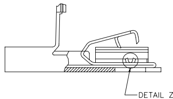
SECTION X-X
