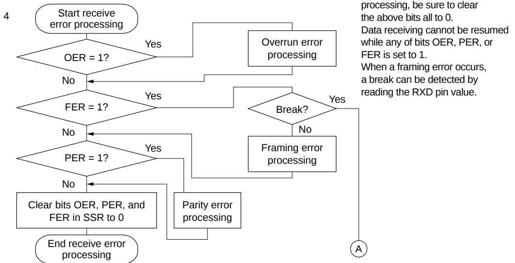
Figure 10.14 Typical Serial Data Receiving Flow Chart in Asynchronous Mode
