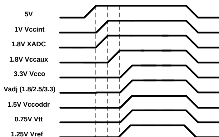
Figure 18 - Power Sequencing
