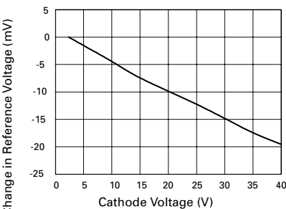
Change in Vref v Cathode Voltage
