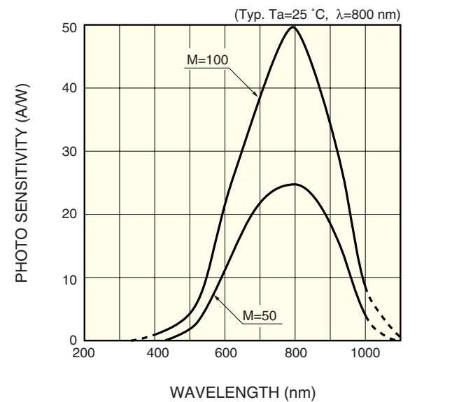
■ Spectral response
