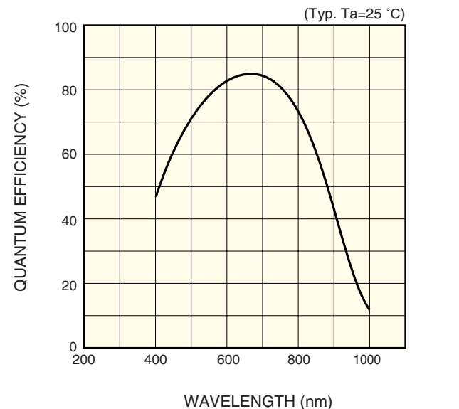
■ Quantum efficiency vs. wavelength
