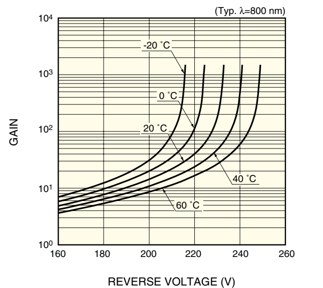
■ Gain vs. reverse voltage
