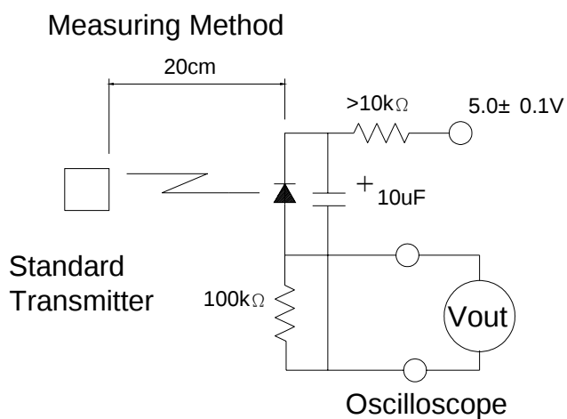
Fig.2 Measuring Method
