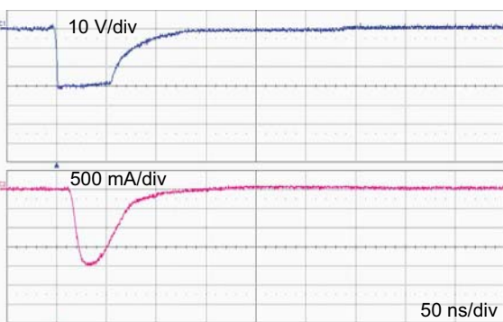
Figure 10. Response to ISO 7637-3 Pulse 3a ( U_s = -150\text{ V} )
