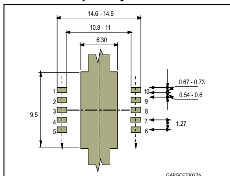
Figure 49. PowerSO-1 pad layout
