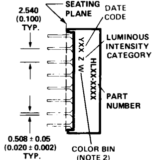
SIDE VIEW E, F, G, H
