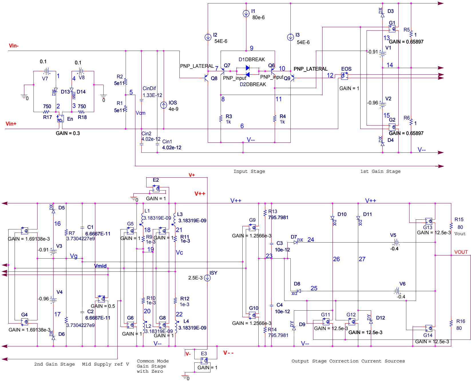
FIGURE 64. SPICE SCHEMATIC
