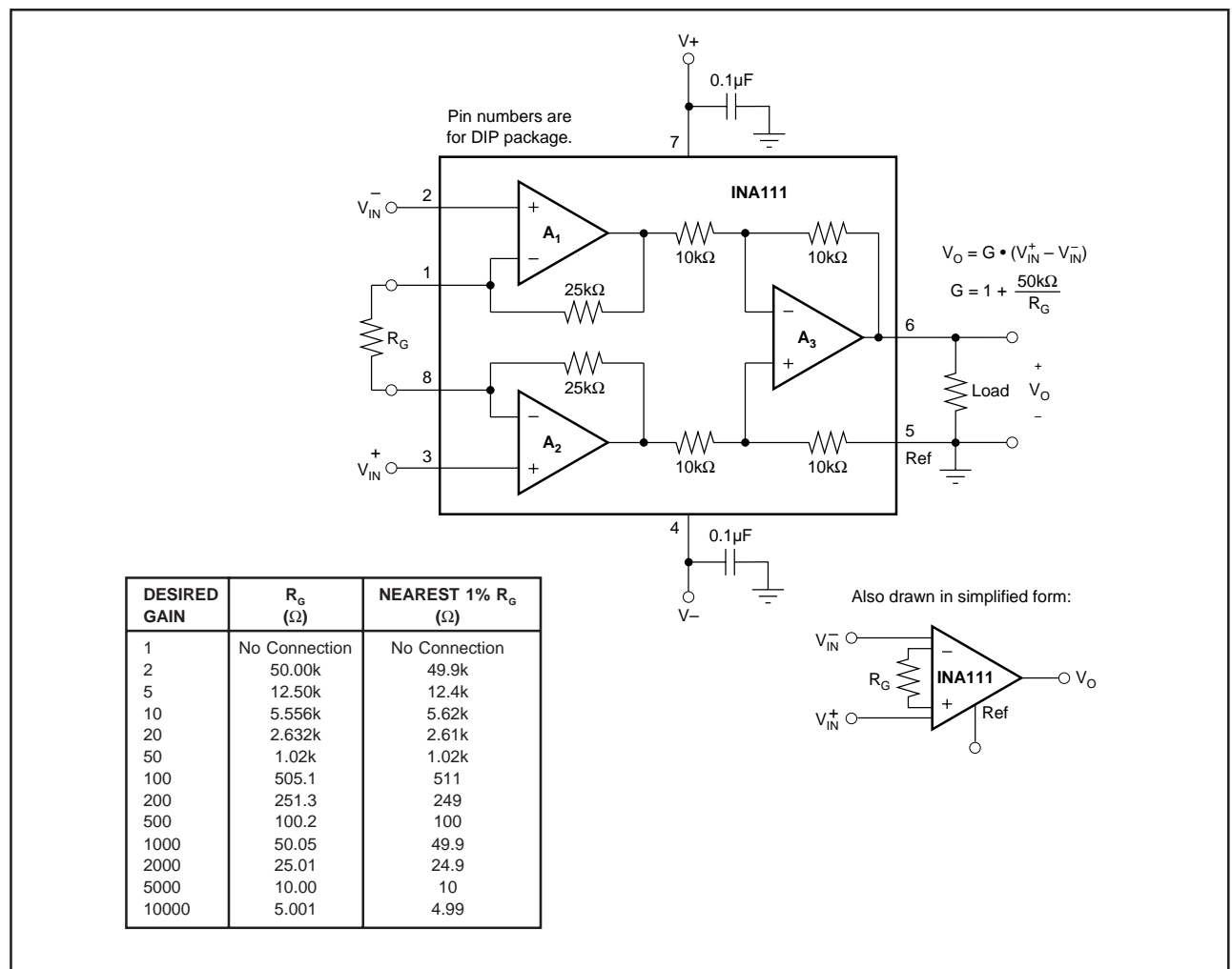
FIGURE 1. Basic Connections
