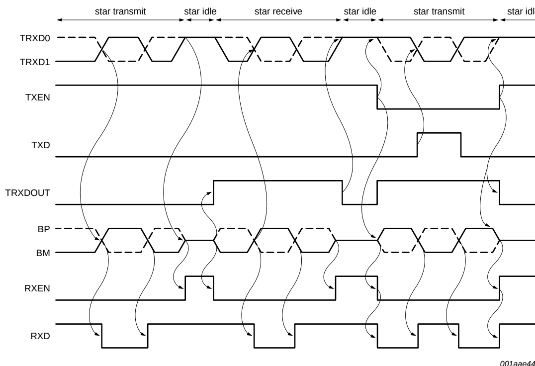
Fig 7. Timing diagram in star configuration
