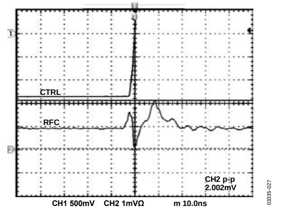
Figure 16. Video Feedthrough
