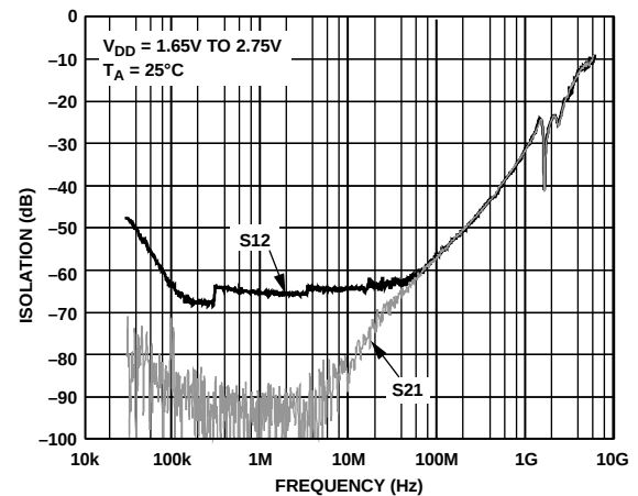
Figure 11. Isolation vs. Frequency over Supplies (RF1/RF2, ADG919)
