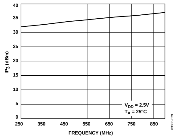
Figure 17. IP3 vs. Frequency
