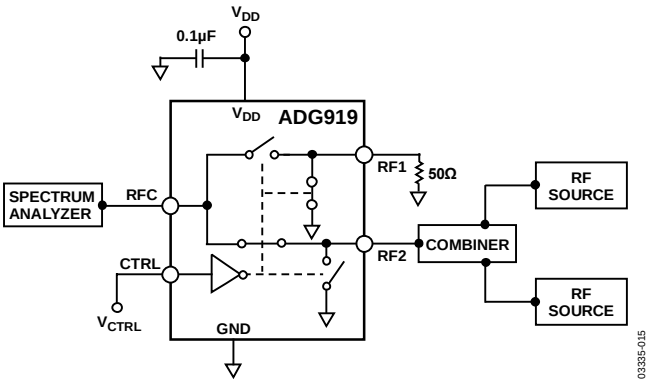
Figure 25. IP_3
