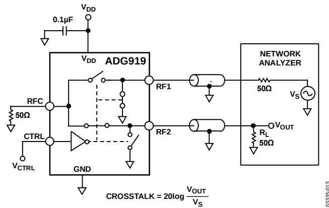
Figure 23. Crosstalk
