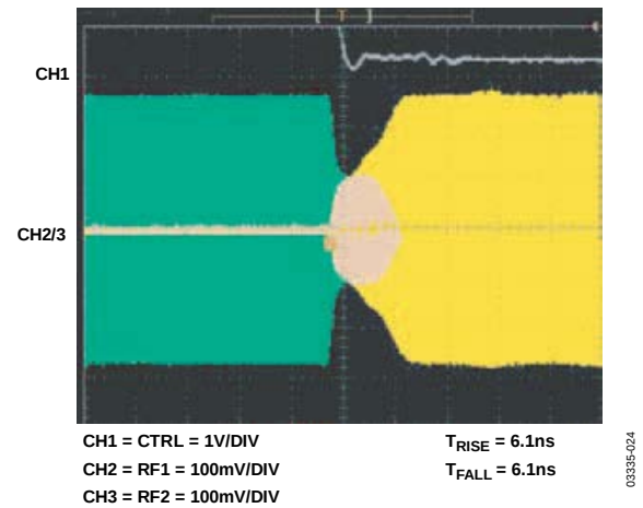
Figure 15. Switch Timing
