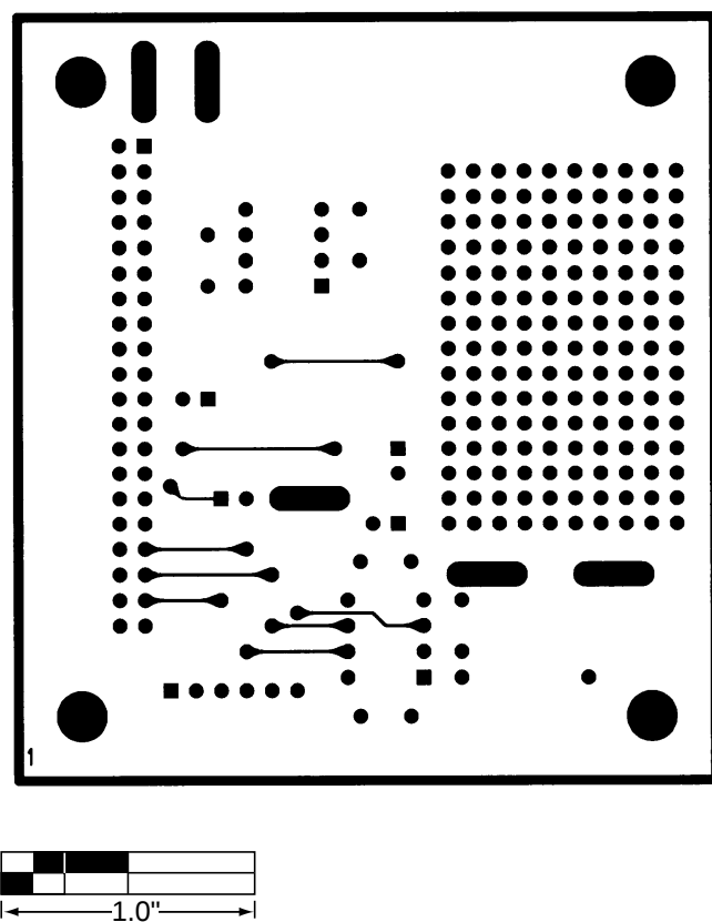
Figure 3. MAX1241 EV Kit PC Board Layout—Component Side
