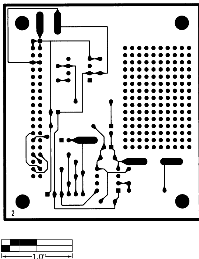
Figure 4. MAX1241 EV Kit PC Board Layout—Solder Side
