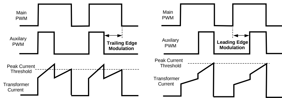
Figure 14. Leading versus Trailing Edge Modulation
