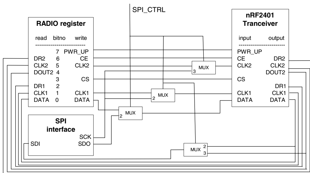
Figure 4-1 : Transceiver interface
