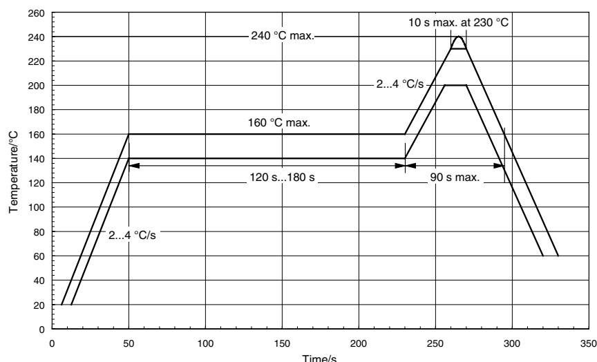
Figure 2. Recommended Solder Profile for Sn/Pb soldering
