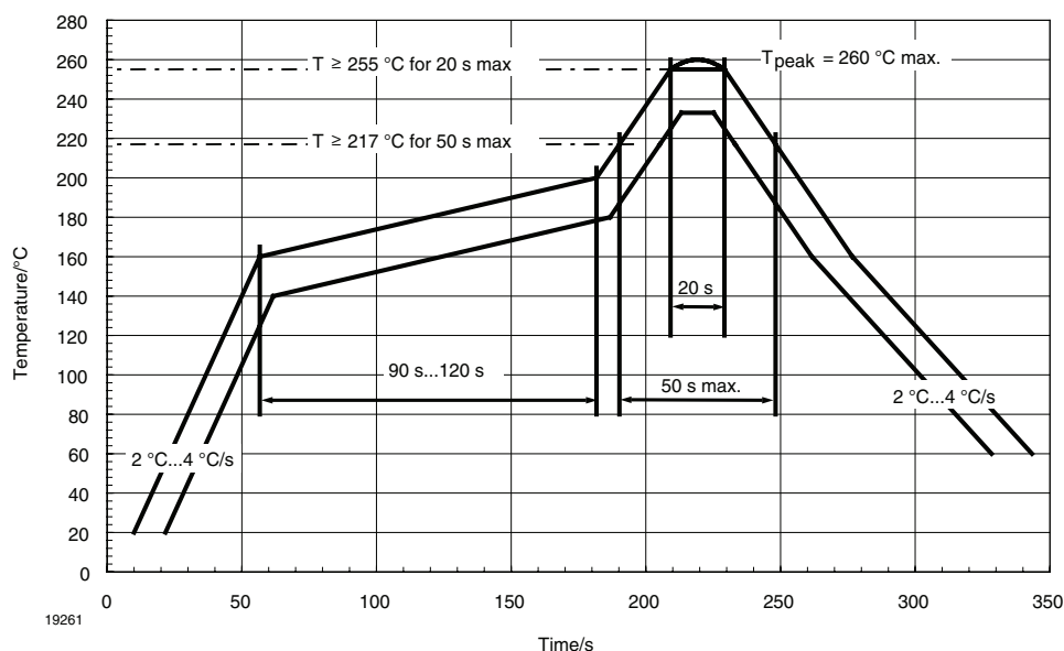
Figure 3. Solder Profile, RSS Recommendation
