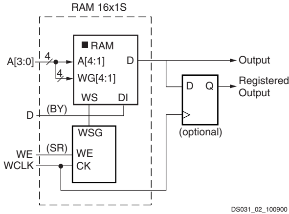
Figure 18: Distributed SelectRAM (RAM16x1S)
