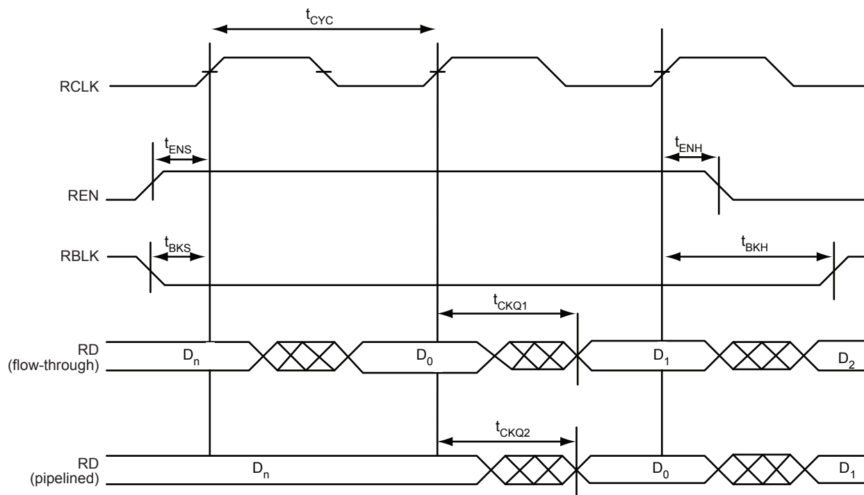
Figure 2-32 • FIFO Read
