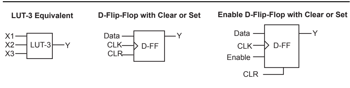
Figure 1-5 • VersaTile Configurations
