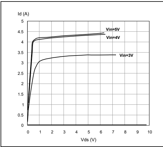
Figure 23. Output characteristics
