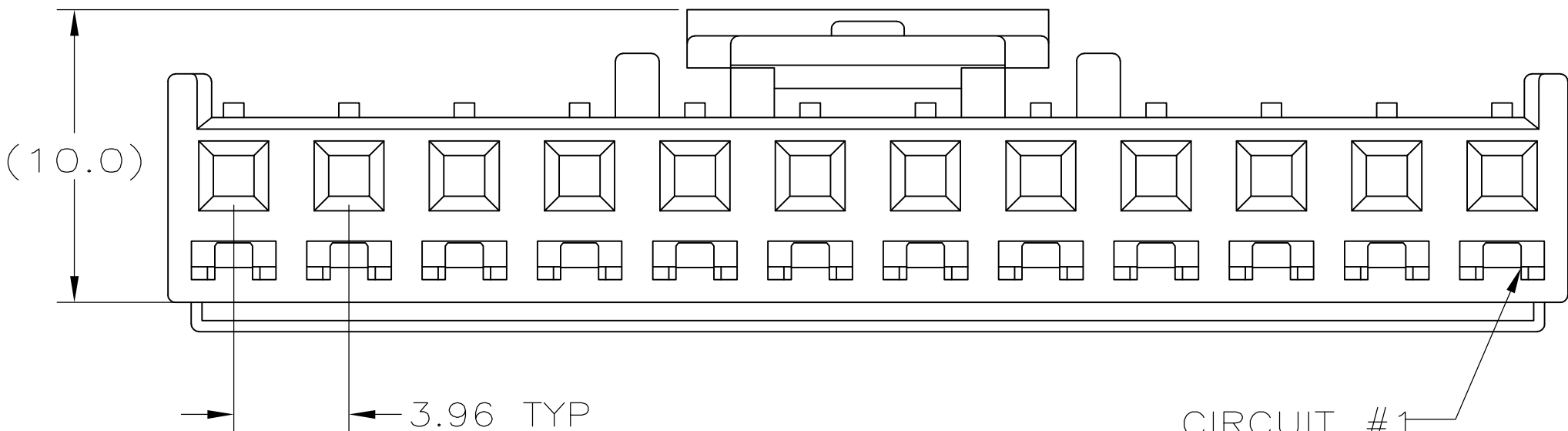
CIRCUIT #1
