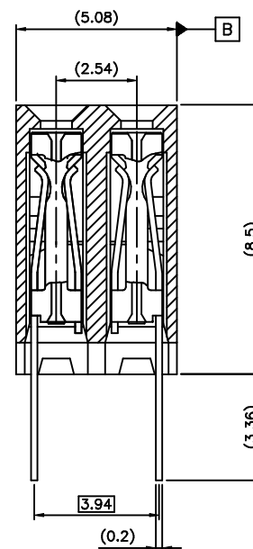
SECTION B-B
