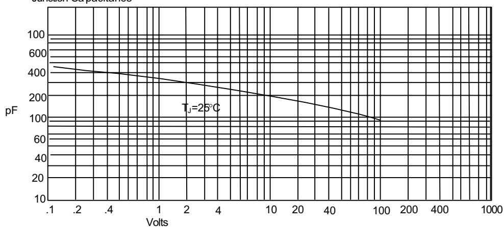
Figure 3 Junction Capacitance
