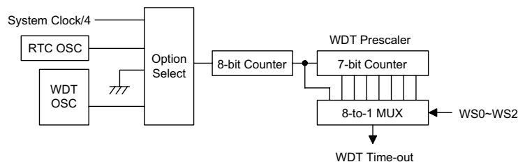
Watchdog Timer
