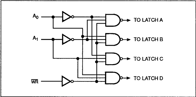
FIGURE 8: Input Control Logic
