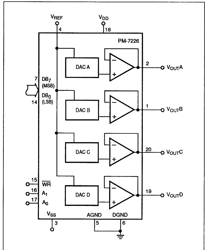
FIGURE 15: Unipolar Operation
