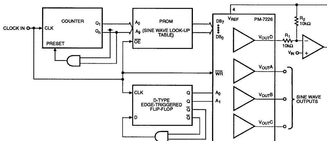
FIGURE 23: 3-Phase Sine Wave Generator Circuit (Using Counter)
