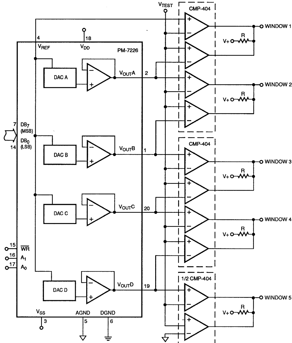
FIGURE 20: Non-Overlapping Window Comparator
