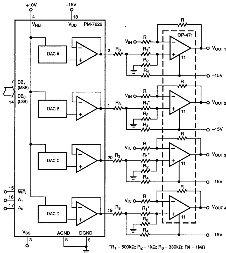
FIGURE 19: Alternate Offset Adjust (See Text)
