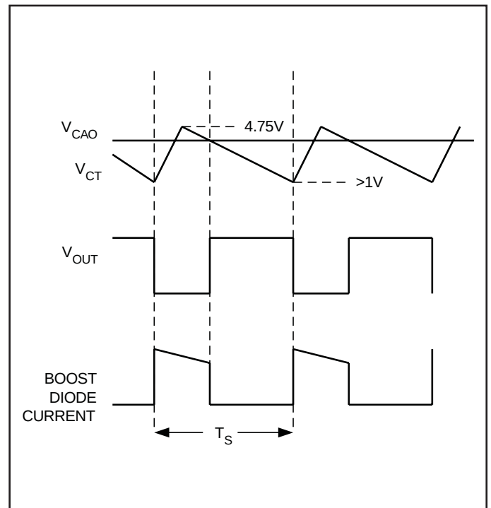
Figure 3b. Oscillator timing waveforms stand alone operation.
