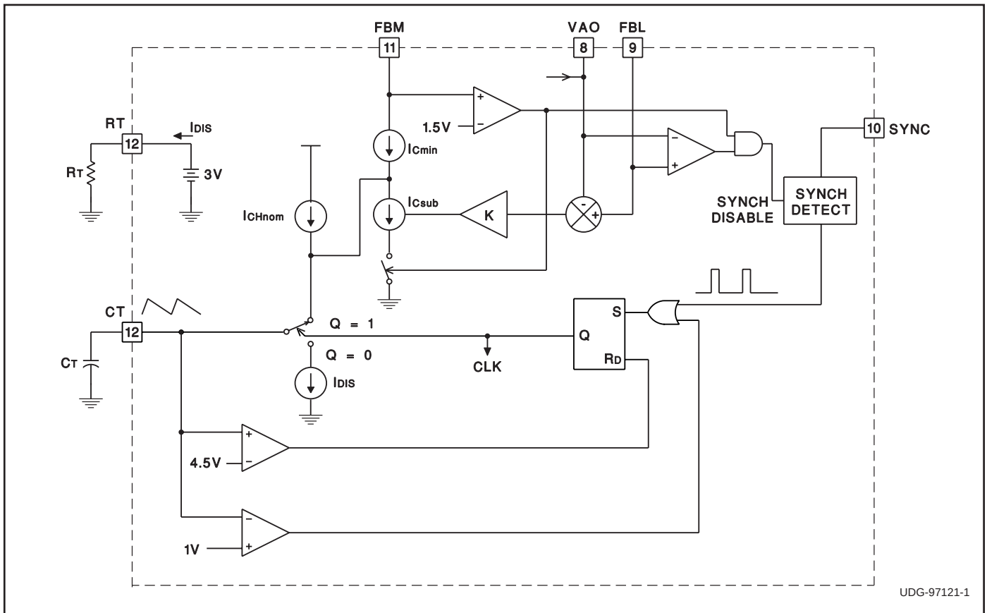
Figure 2. Oscillator block diagram.
