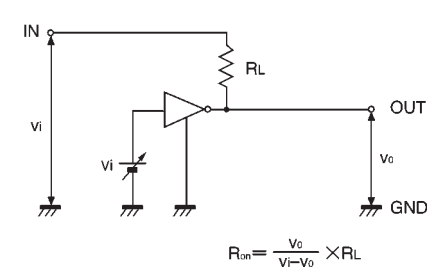
Fig.1 Input "ON" resistance (R on ) measurement circuit
