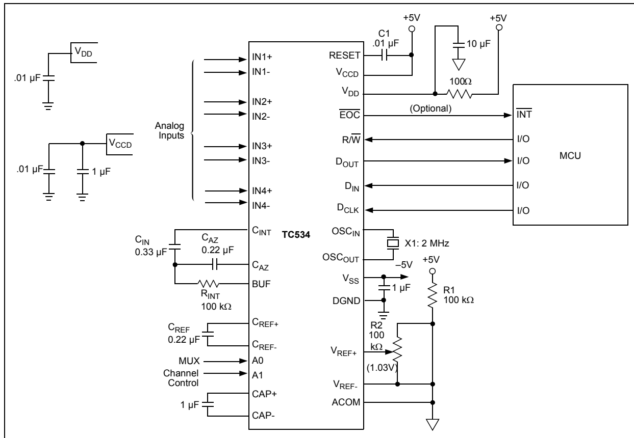
FIGURE 5-1: Typical Application.
