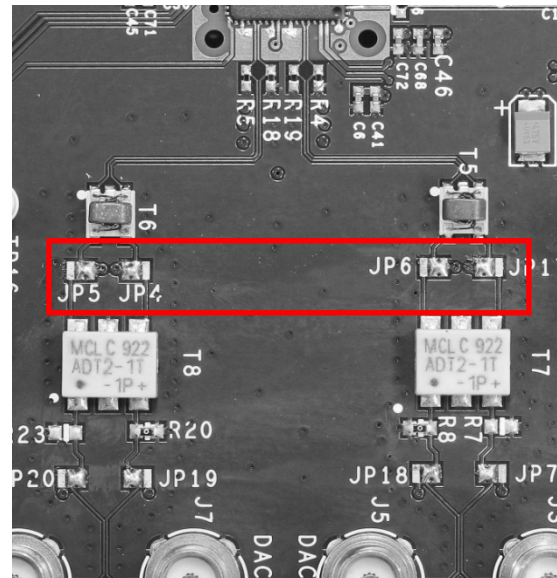
Figure 2 - Modulator Output Configuration
