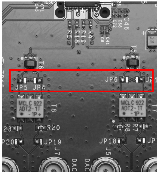
Figure 1 - DAC Output Configuration
