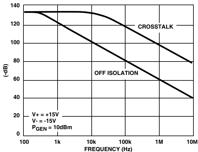
FIGURE 14. CROSSTALK AND OFF ISOLATION vs FREQUENCY
