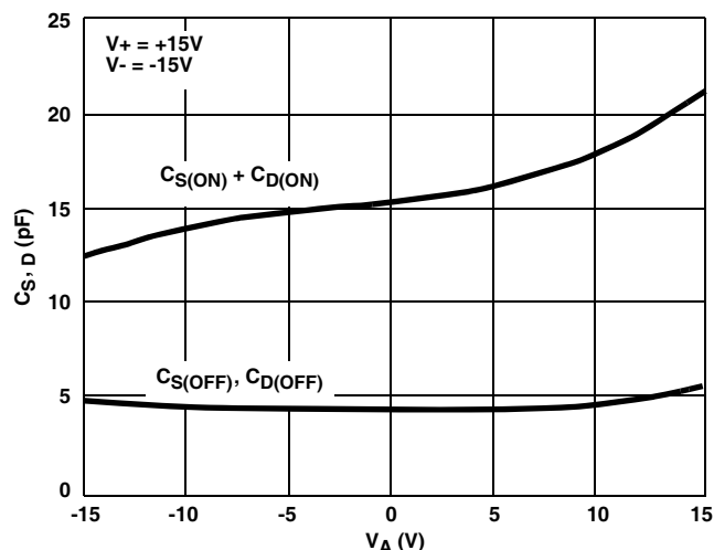
FIGURE 20. SOURCE/DRAIN CAPACITANCE vs ANALOG VOLTAGE
