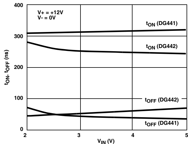
FIGURE 23. SWITCHING TIME vs INPUT VOLTAGE (SINGLE 12V SUPPLY)
