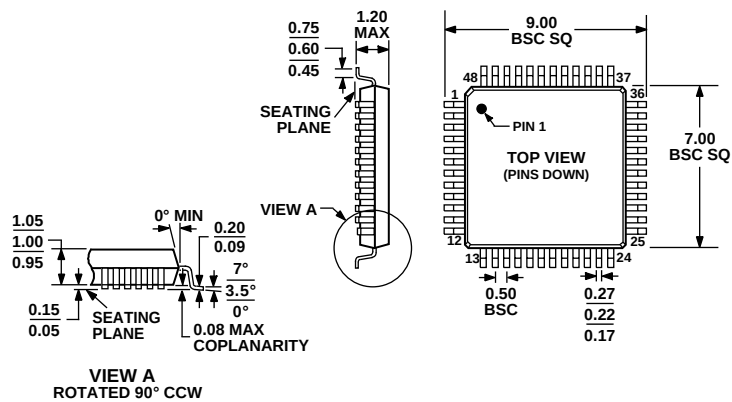
COMPLIANT TO JEDEC STANDARDS MS-026ABC
