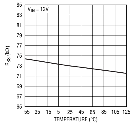
R_{SS} vs Temperature
